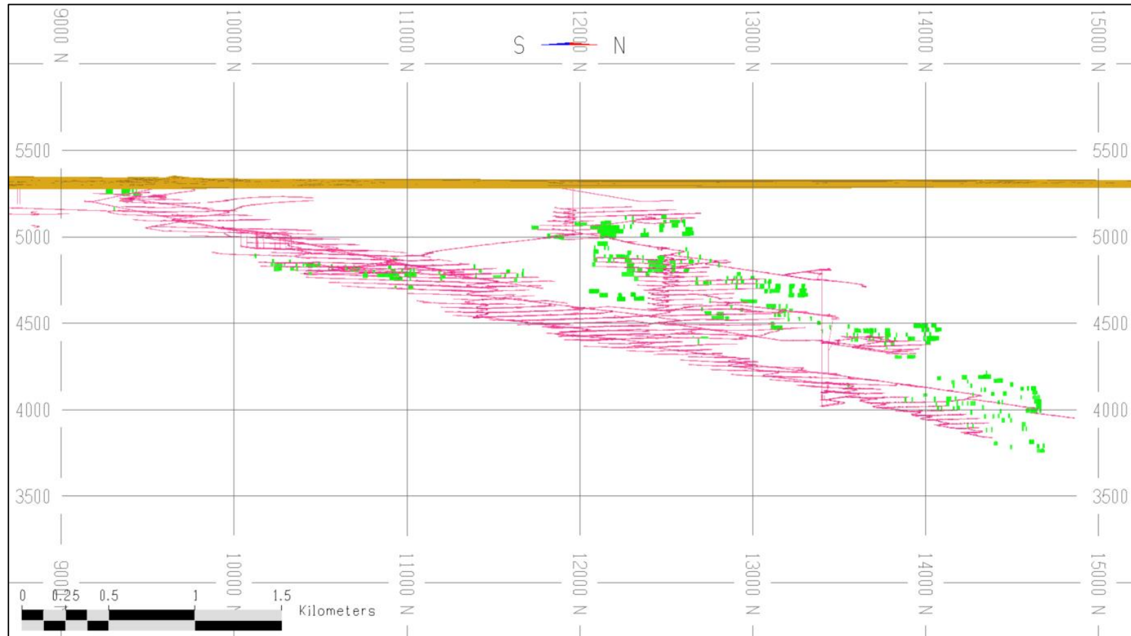
Figure 14.22 – Resource Constraining Underground Reporting Shapes, Longitudinal View (Looking West), Musselwhite Mine
