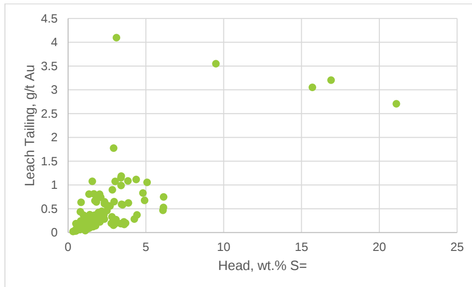
Figure 13.28 – Gold Recovery Variability by Sulfide Grade
