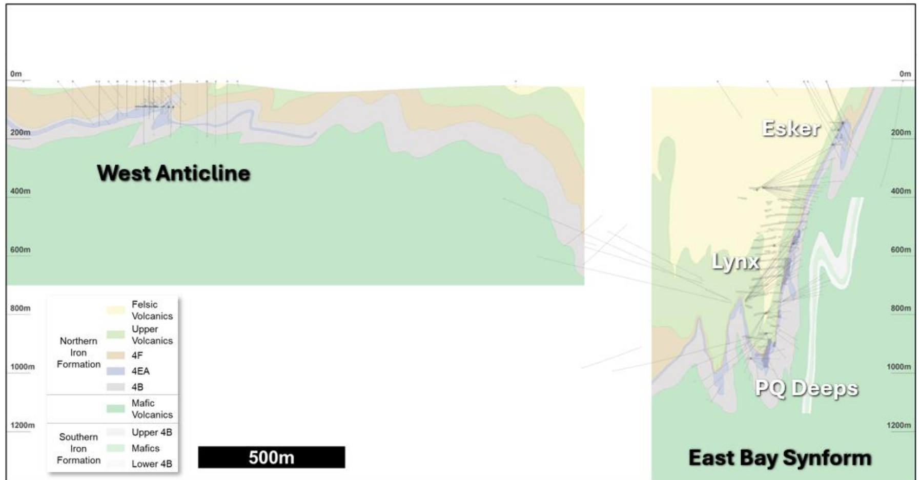
Figure 7.6 – Musselwhite Mine Section 12,500N (Looking North)
