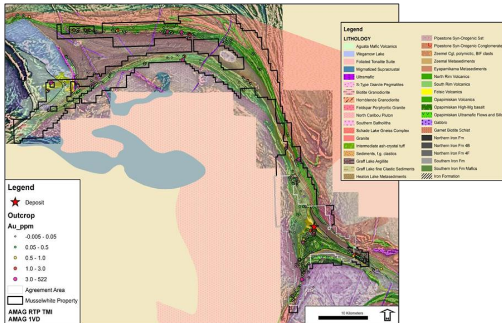
Figure 7.2 – Regional Scale Litho-Structural Interpretation
