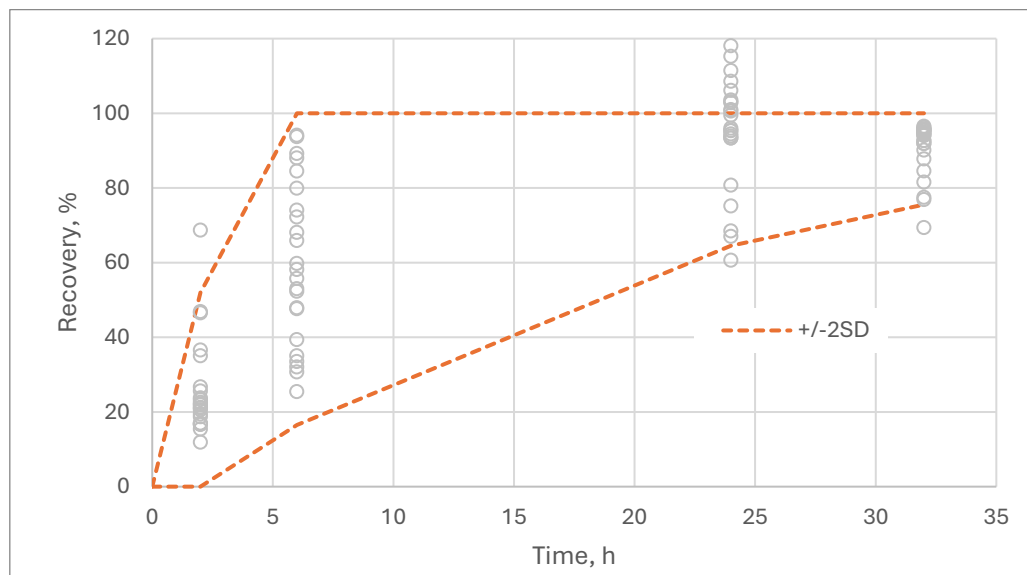
Figure 13.17 –Cyanidation Leach Kinetics, PQD Ext 1
