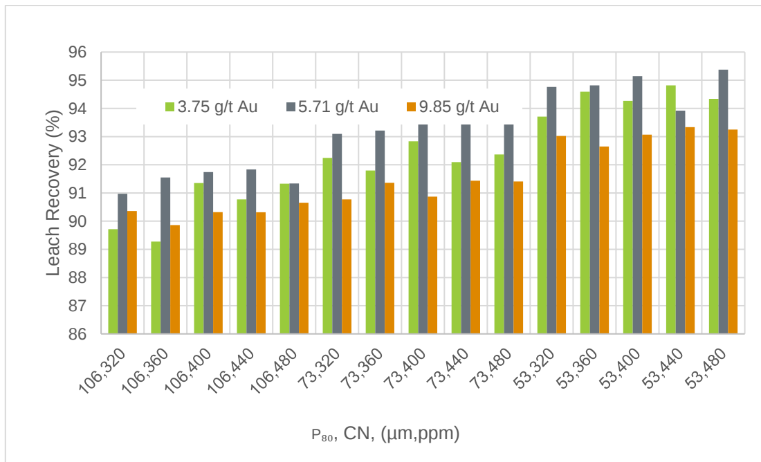
Figure 13.11 – Cyanide Concentration Effects on Recovery, Lynx
